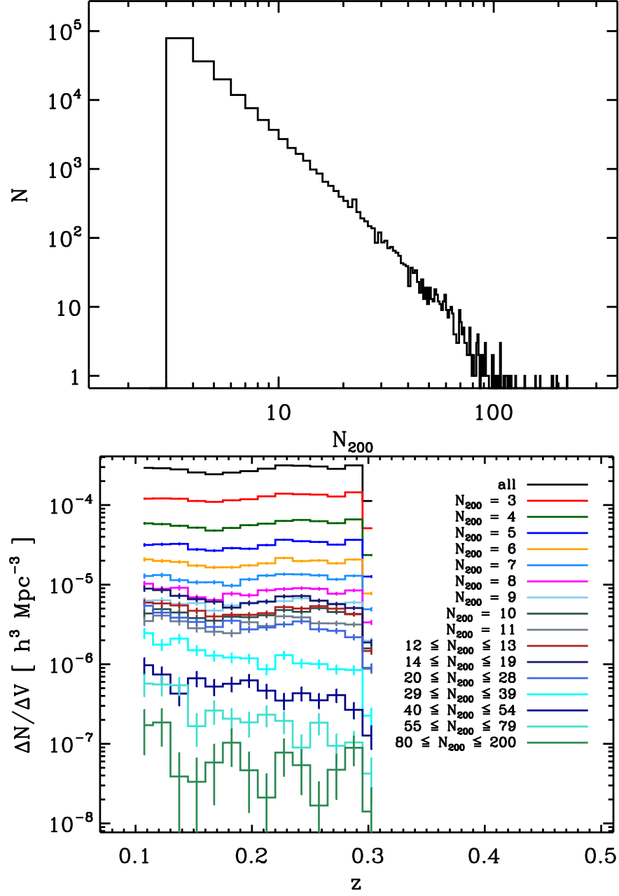
FIG. 4.— Top panel: Histogram of N_{200} , the number of red galaxies brighter than 0.4L_* within r_{200}^{gal} , for the cluster sample. Bottom panel: Number density as a function of redshift for differential bins of N_{200} .
