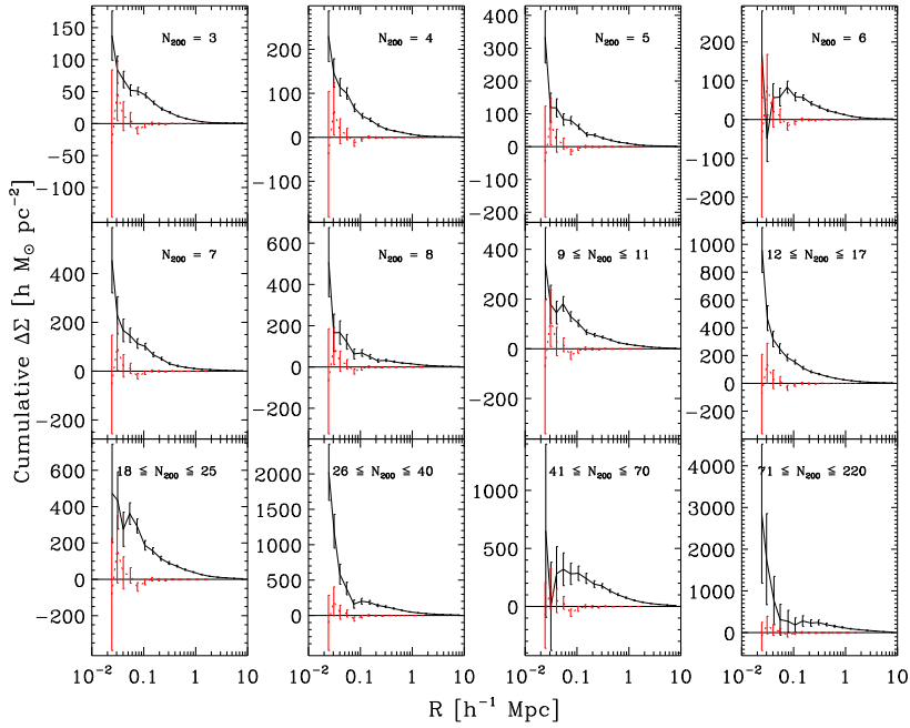
FIG. 13.— Mean estimated contamination of \Delta\Sigma from intrinsic alignments in each of the N_{200} bins, estimated as described in the text. These are cumulative curves so adjacent bins are correlated. In each panel, the intrinsic shear is the red curve and the cluster measurement is the black curve. Note the vertical scale varies between plots.
