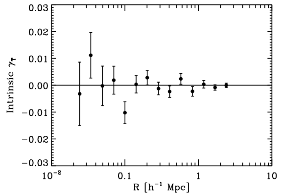
FIG. 12.— Estimate of intrinsic tangential alignments for the spectroscopic cluster sample of (Berlind et al. 2006). The shear tracer population was drawn from the SDSS main spectroscopic sample and chosen to have velocity within \pm 2000 km/s of the cluster. Thus any signal is not due to lensing, but rather intrinsic correlations between galaxy shapes and the tangential direction relative to the lens center. Such an effect would bias the lensing profiles. No net effect was detected.
