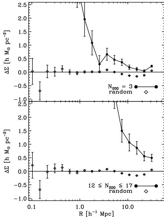
FIG. 5.— Lensing measurement \Delta\Sigma around random points as compared to clusters. The top panel compares randoms to clusters for the N_{200}=3 bin; the bottom panel shows the 12 \leq N_{200} \leq 17 bin. The non-zero detection at large scales is indicative of residual additive systematics in the PSF correction. The random signal dominates on large scales for the relatively low signal bin shown in the top panel. The contamination is less important but still significant for the intermediate bin shown in the bottom panel. The random signal is subtracted from the cluster signal for all samples presented in this work.
