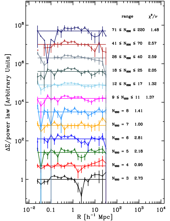
FIG. 8.— Power law fits in each N_{200} bin. For each bin, the best fitting power law (see Table 1) has been divided out and the signal scaled arbitrarily to separate the profiles visually. For clarity, the error bars for points with S/N < 1 have been suppressed for the top two bins. Each curve is labeled by its richness range and reduced \chi^2 for the power law fit. The profiles are not generally good fits to a power law and demonstrate systematic deviations as a function of scale.
