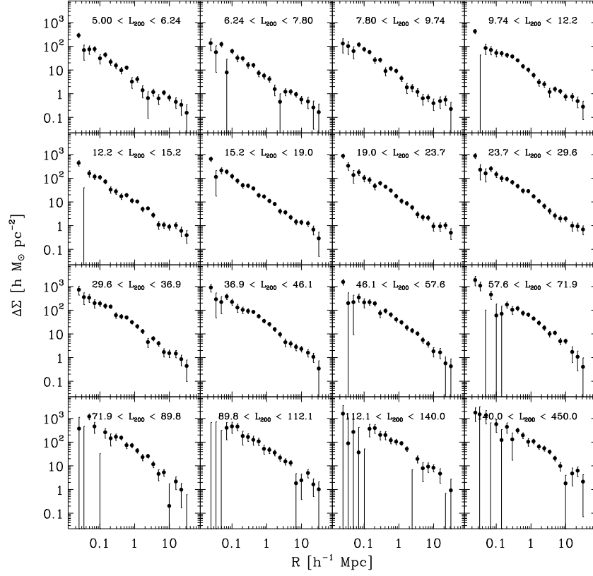
FIG. 10.— Same as Figure 7 but in 16 bins of L_{200} , the total i-band luminosity of ( > 0.4L_* ) galaxies within r_{200}^{gals} .
