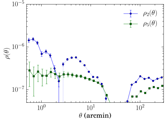
Figure 9. The \rho statistics for the PSF shape residuals. Negative values are shown in absolute value as dotted lines. Requirements on the \rho statistics are specific to individual science cases.
