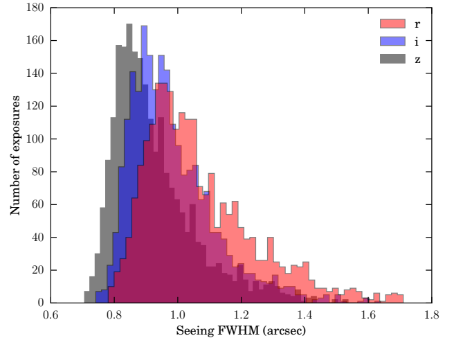
Figure 6. The distribution of the median seeing FWHM of the stars used to model the PSF in the riz -bands. The median seeing of these distributions is 1''.03 in the r -band, 0''.95 in the i -band, 0''.89 in the z -band, and 0''.96 in the three bands overall.
