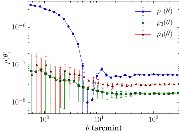
Figure 9. The \rho statistics for the PSF shape residuals. Negative values are shown in absolute value as dotted lines. Requirements on the \rho statistics are specific to individual science cases.
