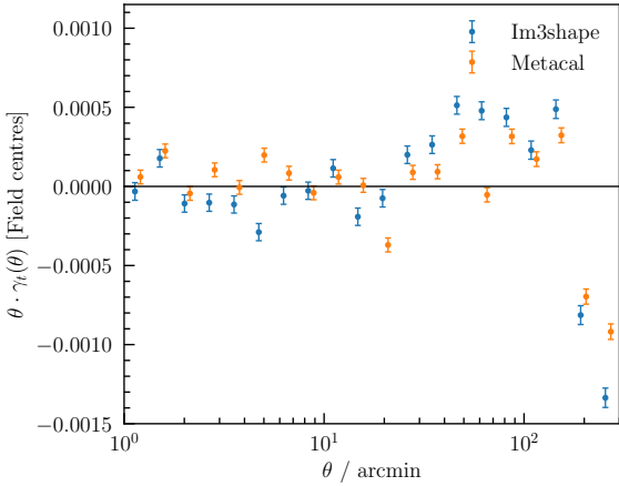
Figure 17. The tangential shear of galaxies in the two catalogues around field centres, after subtraction of shear around random points.
