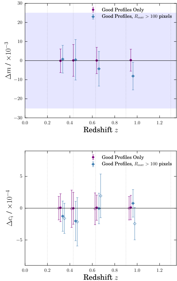
Figure A2. Change in the multiplicative bias (top) and additive bias (bottom) after removal of bad COSMOS profiles, relative to the value derived using all galaxies. In the lower panel the filled markers show the c_1 component and the open ones show c_2 .
